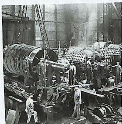
1906, atelier turbines
